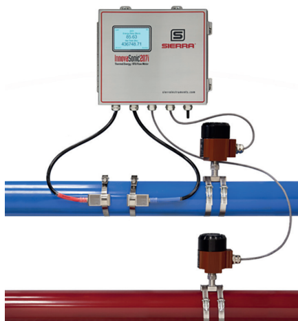
Sierra Instrument's clamp-on ultrasonic liquid/thermal BTU flowmeter
